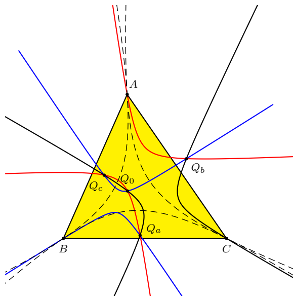
Figure 8. Pencil of hyperbolas with four real intersections
