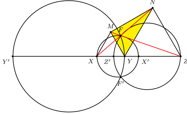
Figure 13. Coaxial circles with diameters XX' , YY' , ZZ'
