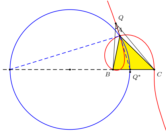
Figure 2. The cubic \mathcal{H}_a and the A -Apollonian circle
