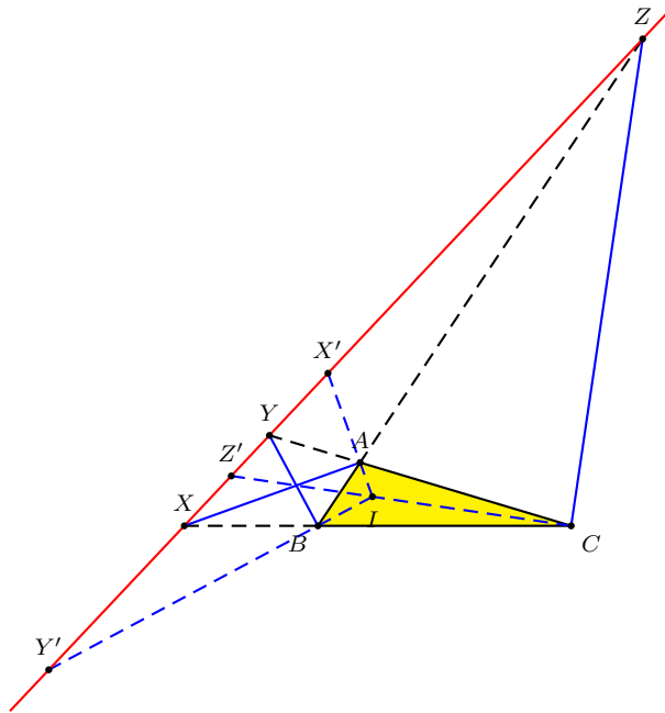
Figure 12. The external angle bisectors problem
