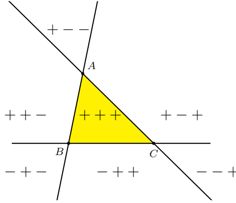
Figure 6. Partition of the plane by the sidelines of a triangle
