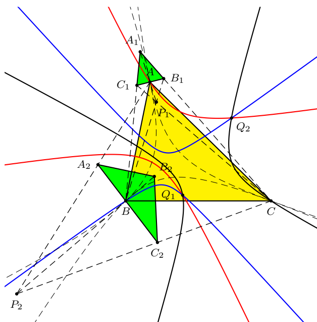
Figure 10. Pencil of hyperbolas with two real intersections
