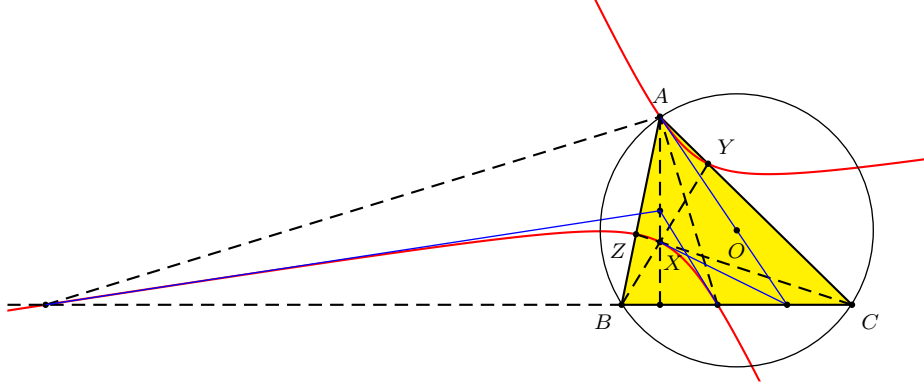
Figure 5. The hyperbola \mathcal{C}_a
