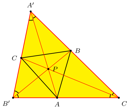
Figure 1. The angle bisectors problem
