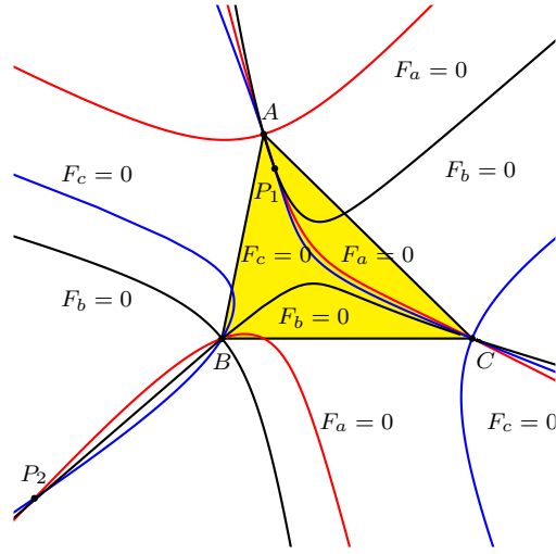
Figure 3. The cubics F_a = 0 , F_b = 0 and F_c = 0
